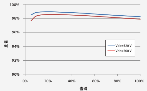
Efficiency Curve / 효율곡선
